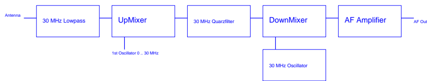
Principle of DRM Demonstration Receiver
